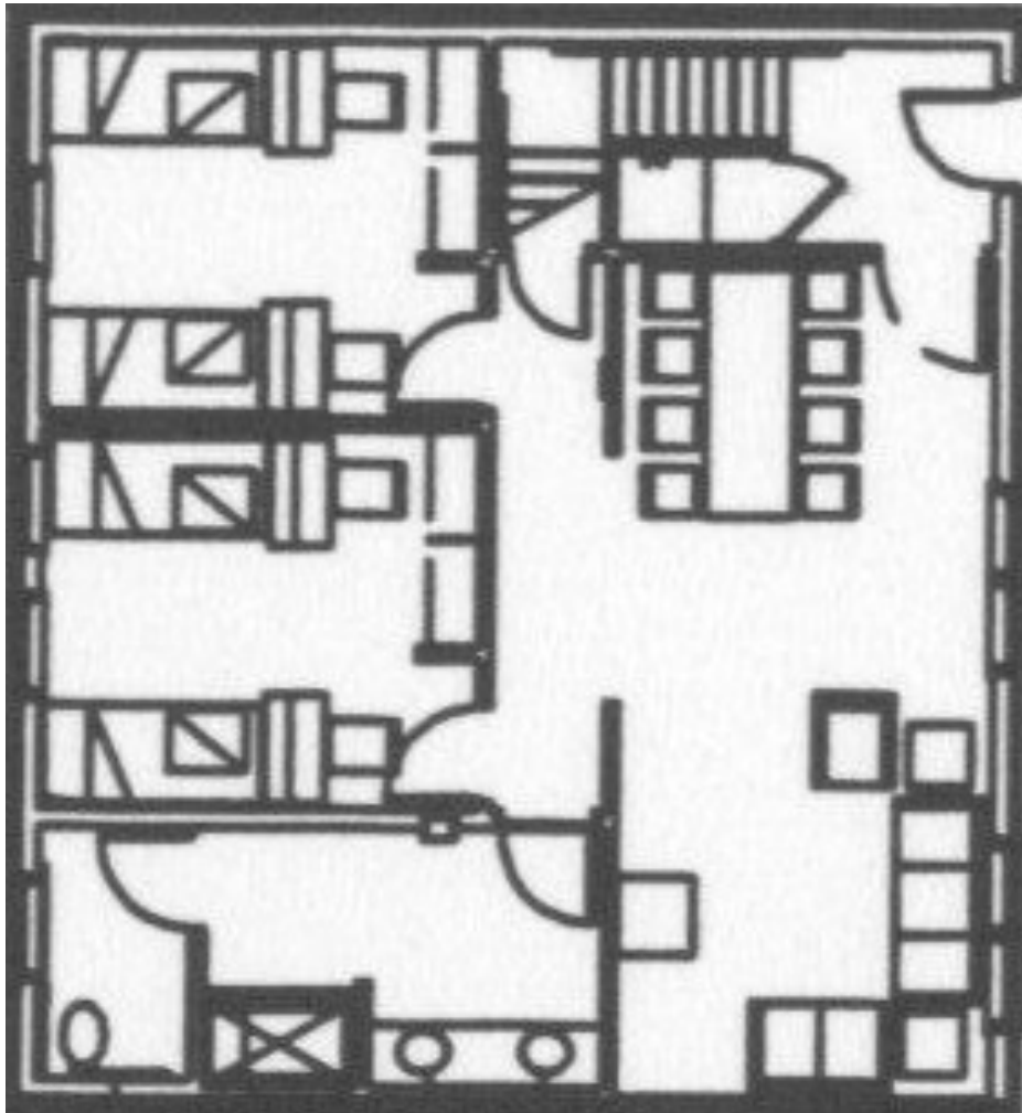
1st Floor
