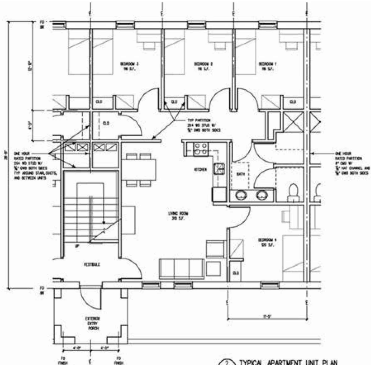
2 TYPICAL APARTMENT UNIT PLAN SCALE 1/4" = 1'-0"
