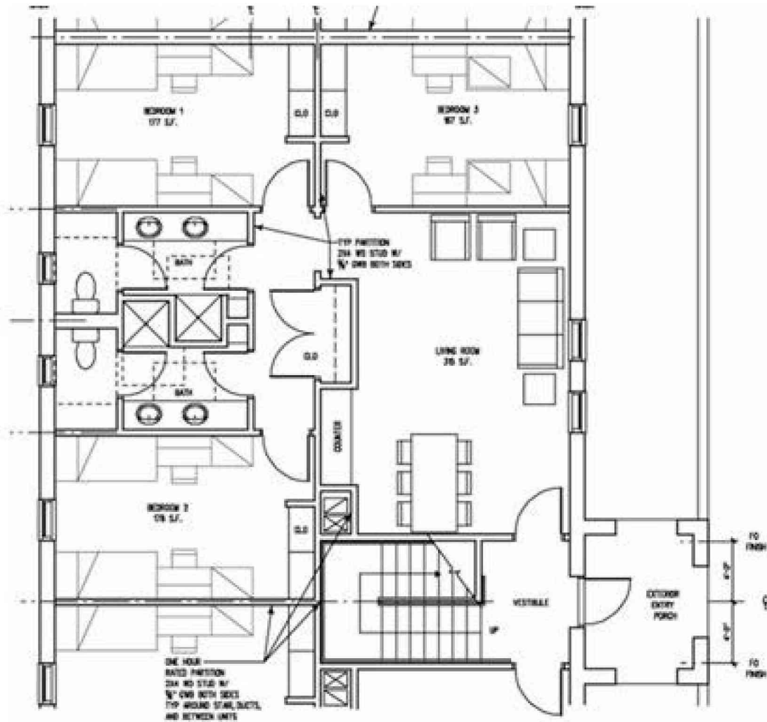
2 A1.3 TYPICAL SUITE UNIT PLAN SCALE 1/4" = 1'-0"
