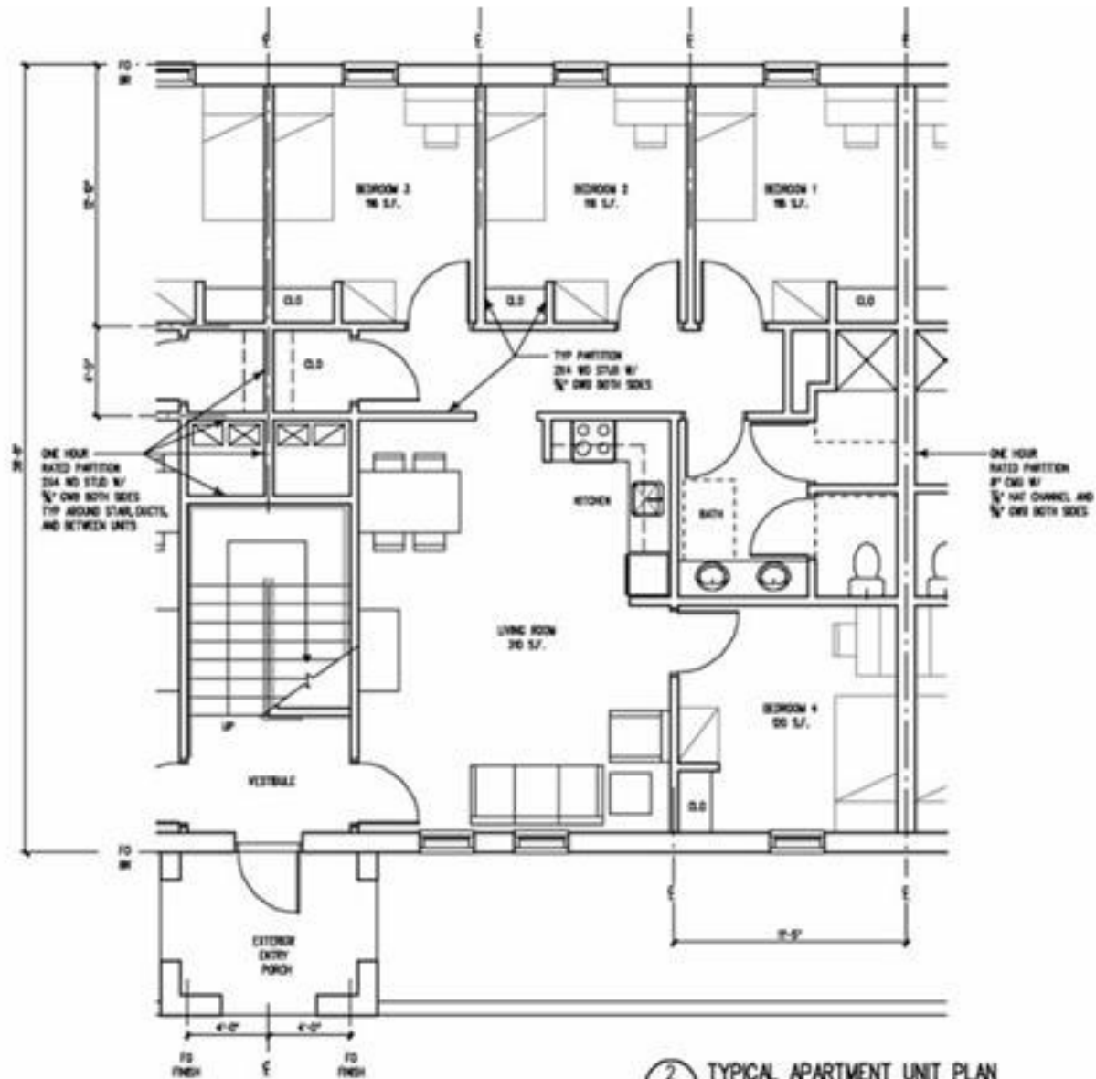
2 TYPICAL APARTMENT UNIT PLAN A.B.1 SCALE: 1/4" = 1'-0"
